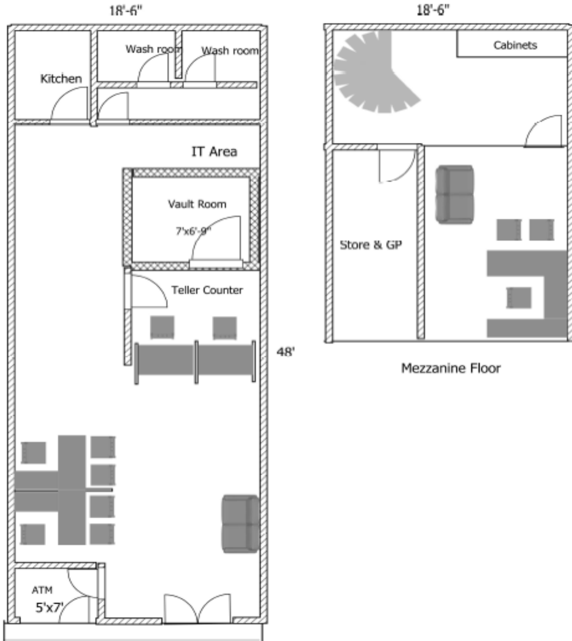
PROPOSED Nankana Sahib Branch Relocation Ground Floor
