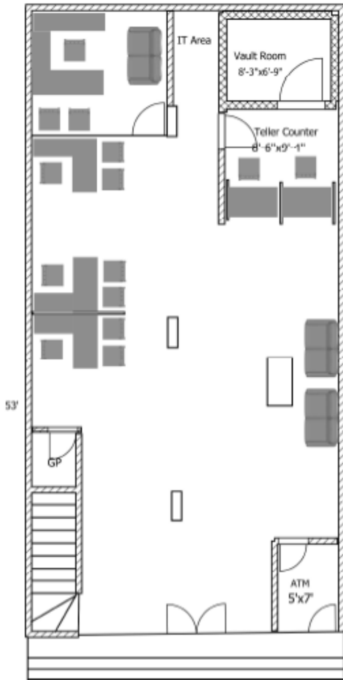
Ground Floor PROPOSED ALIPURCHATTA BRANCH Relocation
