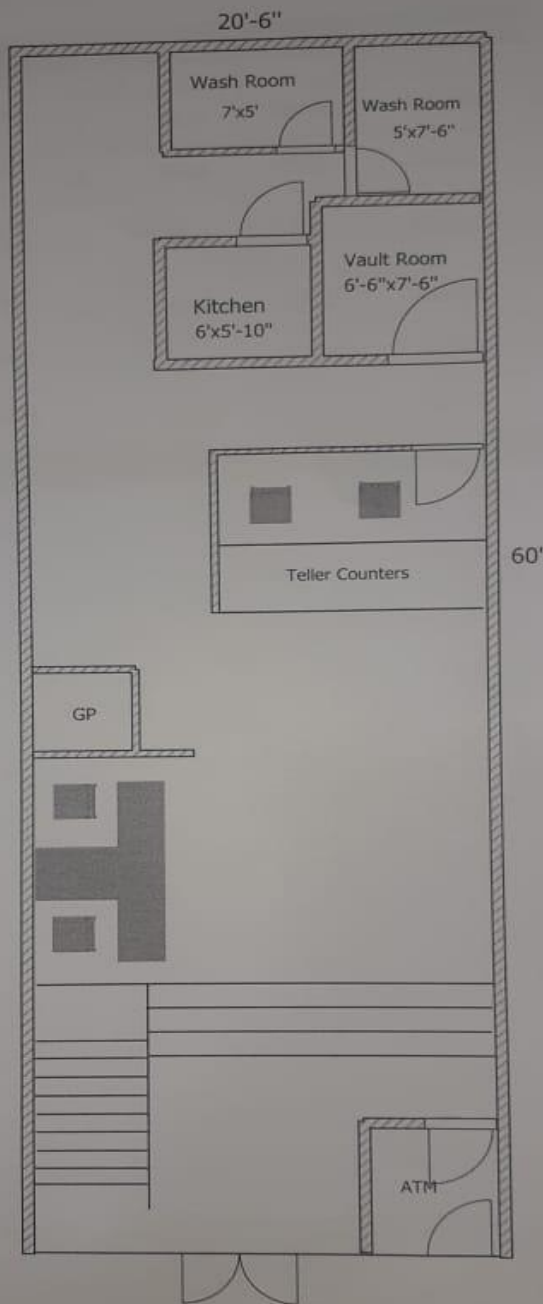
Layout Plan Haider Road Br Rawalpindi Ground Floor
